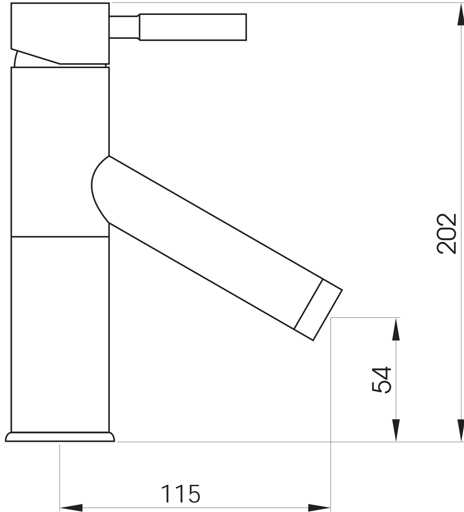
A2-102 Basin Mixer
