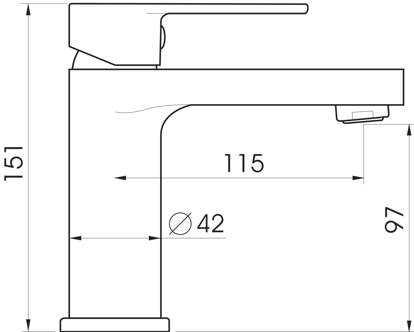
AZ-101 Basin Mixer
