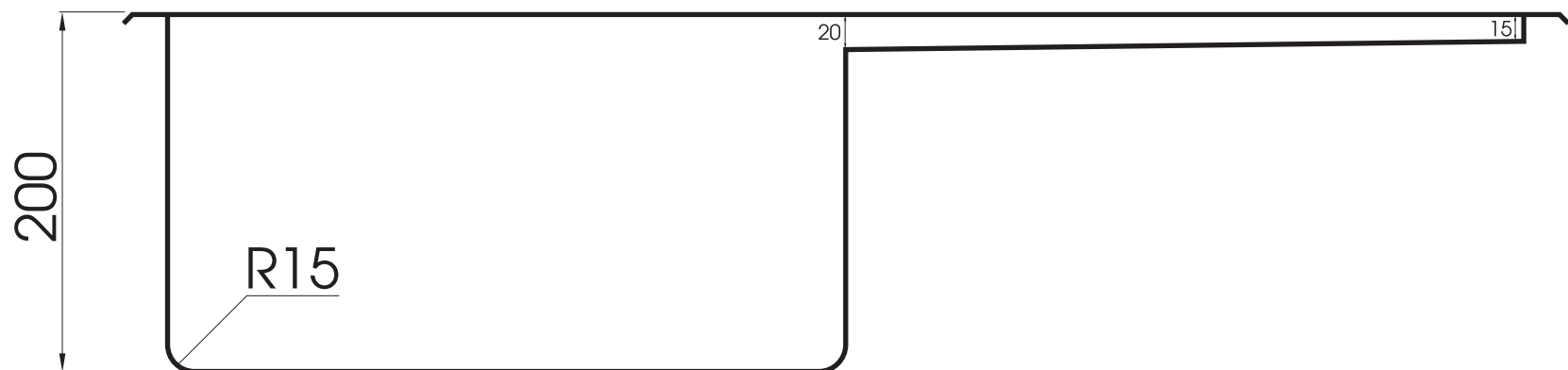
TKS-110R Single Bowl Under mount or Inset
