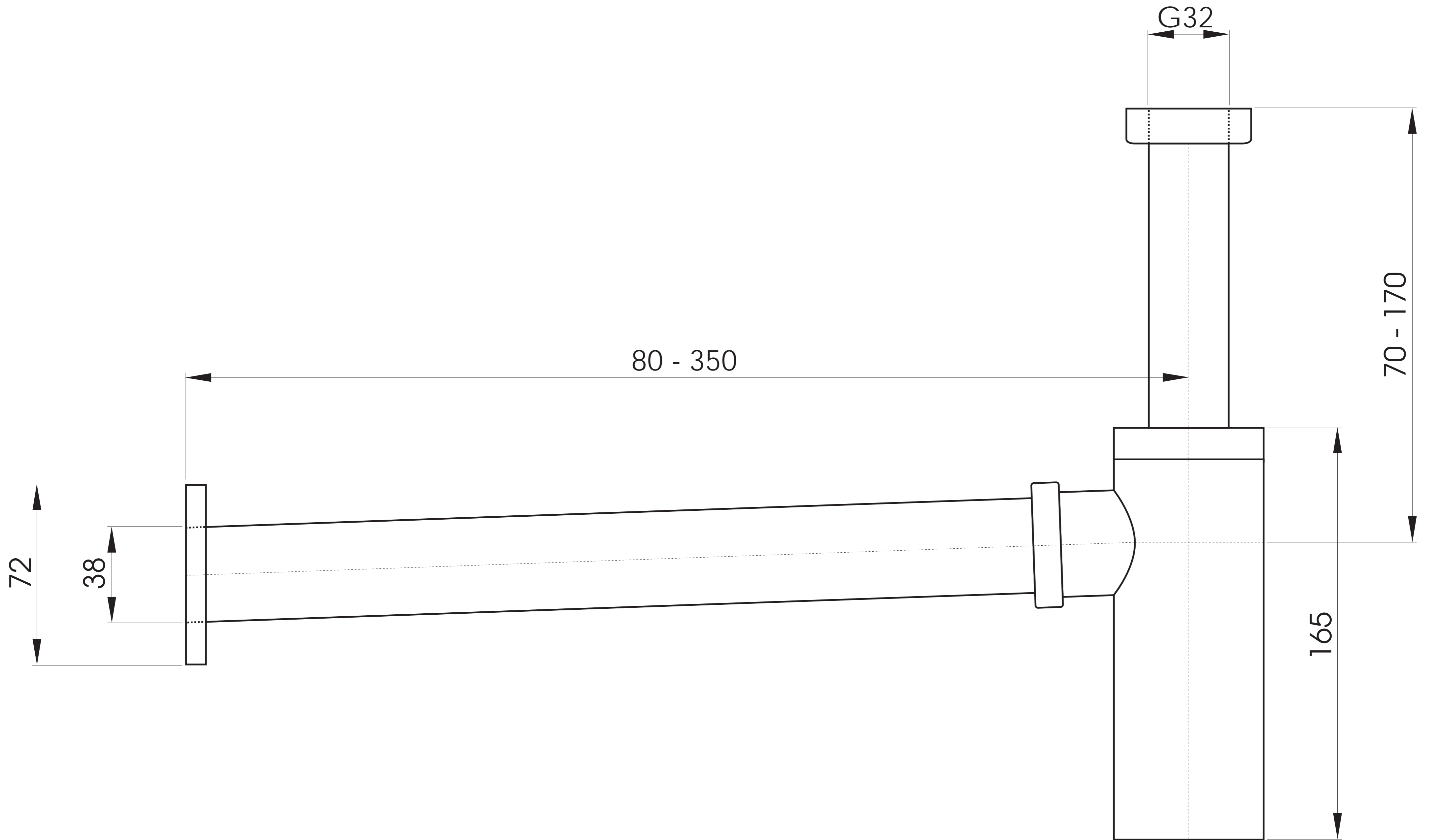
BTB-141 Slim-Line Bottle Trap
